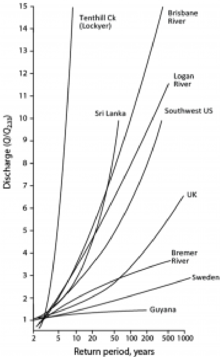
Figure 2. Flood growth curves for selected regions around the world compared to rivers in the Moreton Bay catchment (35, 36).
