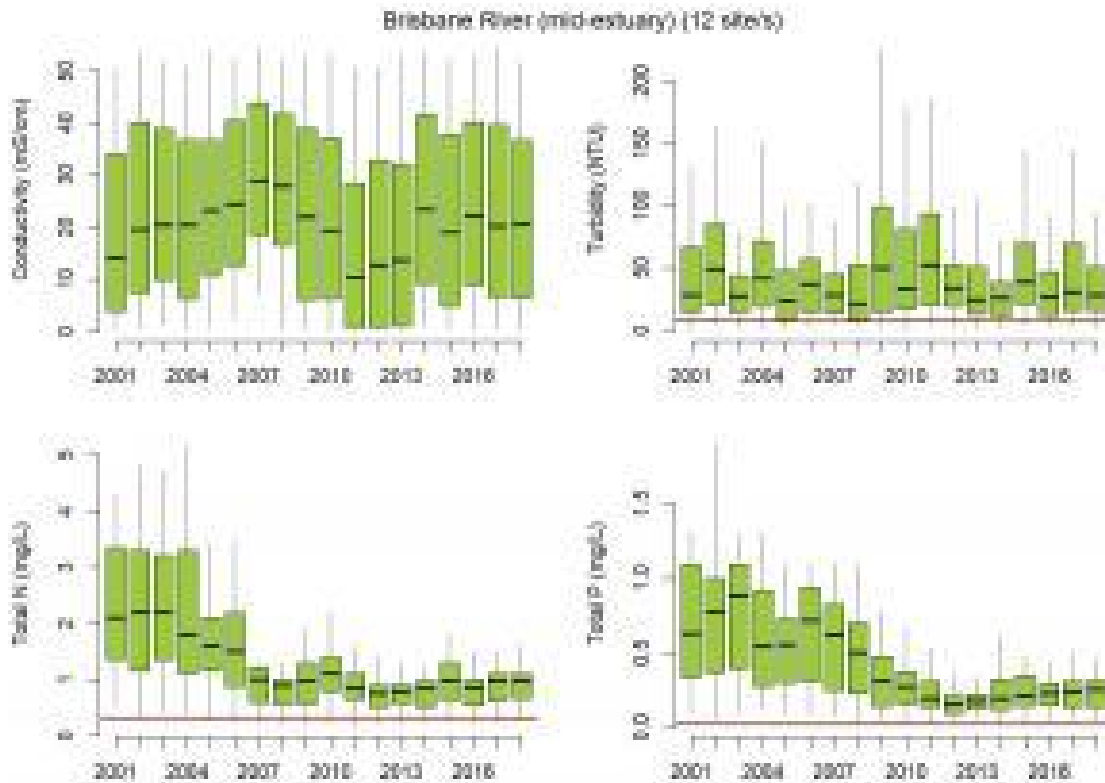
Figure 9. Box and whisker plots for 12 mid-estuary Brisbane River sites as per Fig. 7.
