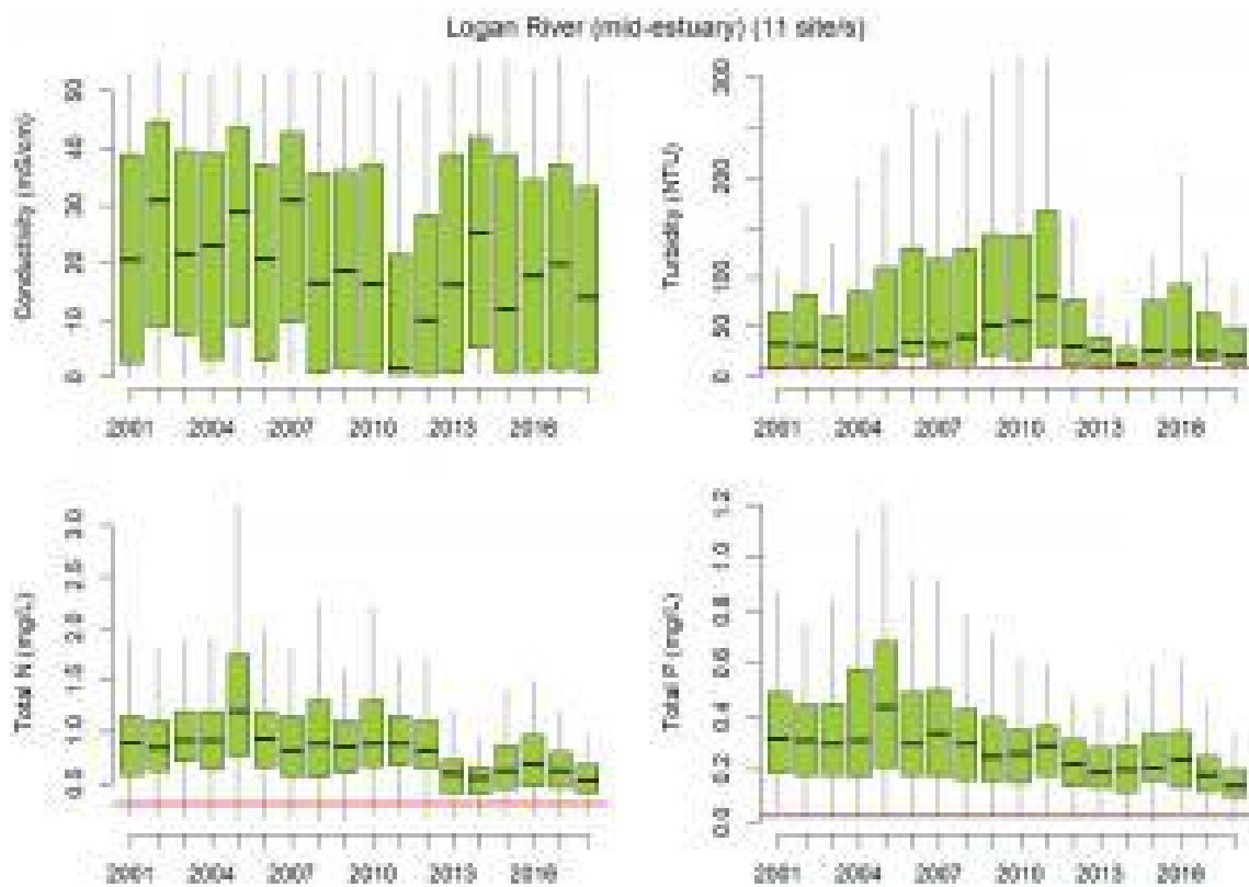
Figure 10. Box and whisker plots for 11 mid-estuary Logan River sites as per
