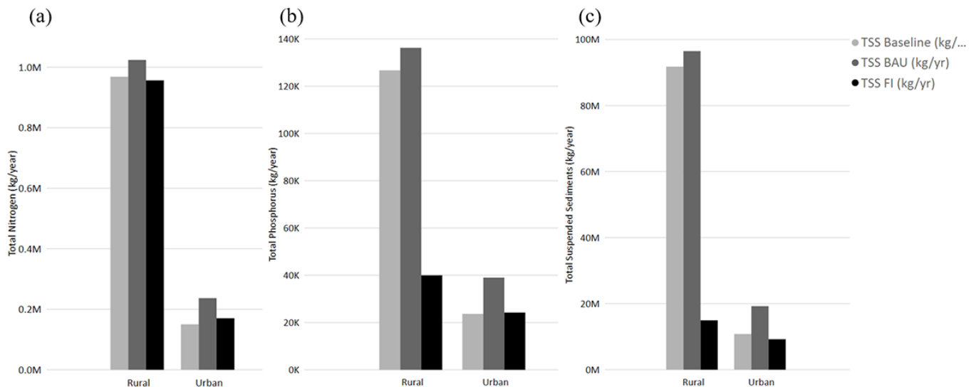
Figure 12. Pollutant loads (kg/year) under three management scenarios. Results of pollutant load generation modelling for the Moreton Bay catchment, recreated from Healthy Land and Water (28). Two future land-use management scenarios are compared with existing practices. Baseline 2015 (light grey bars) – current land management practices and existing land uses; Business-As-Usual (dark grey bar) – current land management practices, with increased population and expanded urban footprint at 2030; Full Investment (black bars) as
