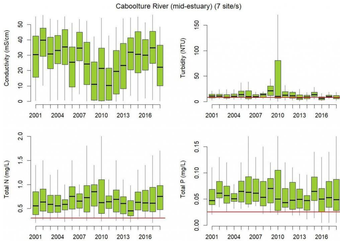
Figure 7. Box and whisker plots for 7 mid-estuary Caboolture River sites showing annual median, upper and lower quartile for conductivity (mS/cm), turbidity (NTU), total nitrogen (mg/L), total phosphorus (mg/L) for the financial years (July to June) 2001 to 2018. Red lines represents Queensland Government’s water quality objectives as shown in Table 1.
