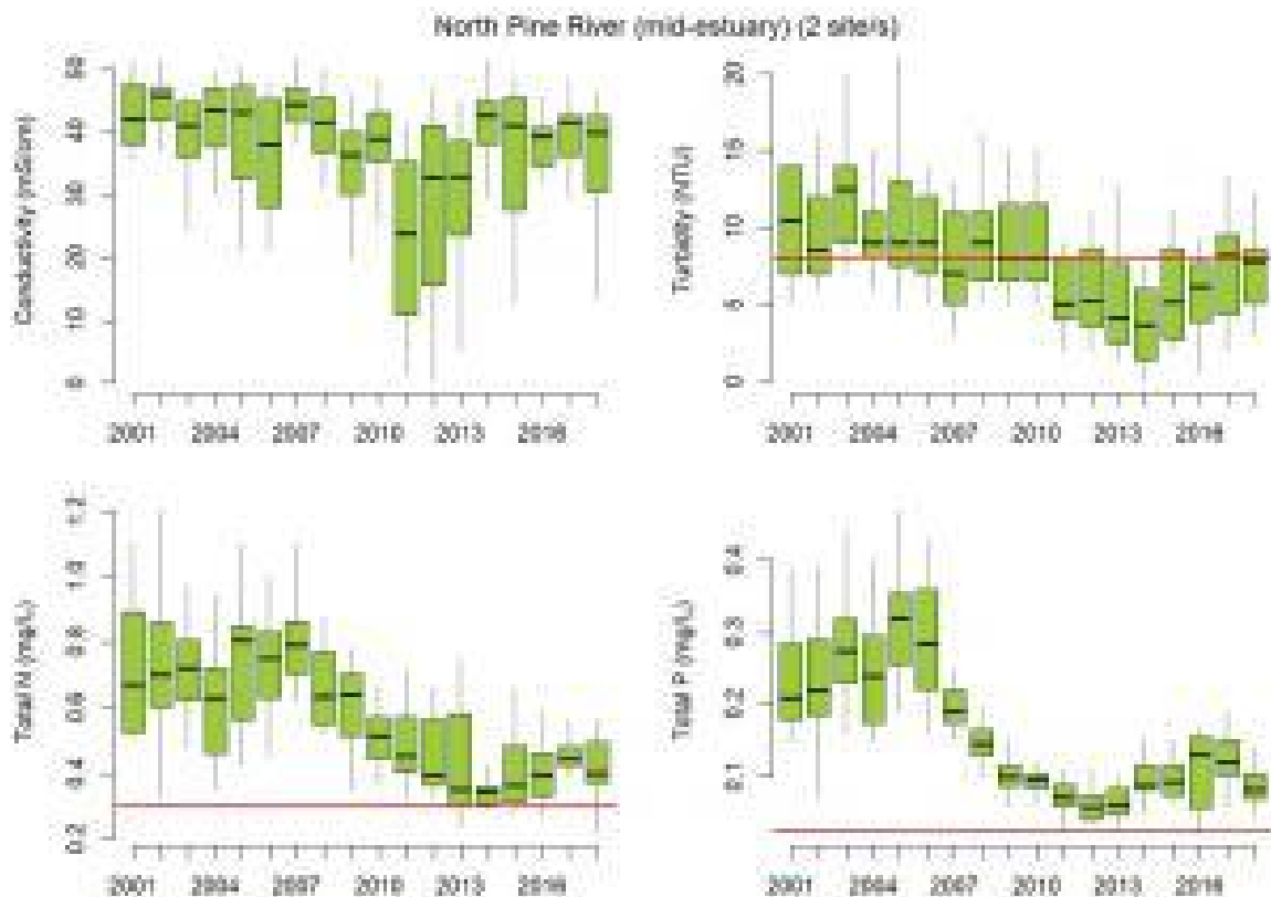
Figure 8. Box and whisker plots for 2 mid-estuary North Pine River sites (see Fig. 7 for explanation).
